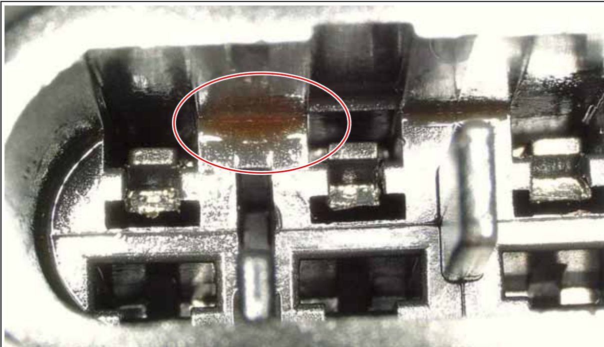
Figure 1 oil contaminated plug housing
