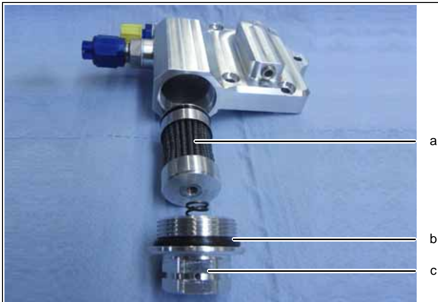
Fig. 6.46 Gearbox oil filter assembling
