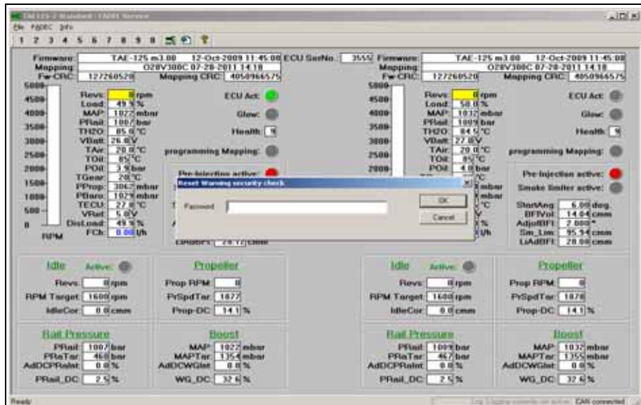
Fig. 6.39 FADEC read-out - Enter password
