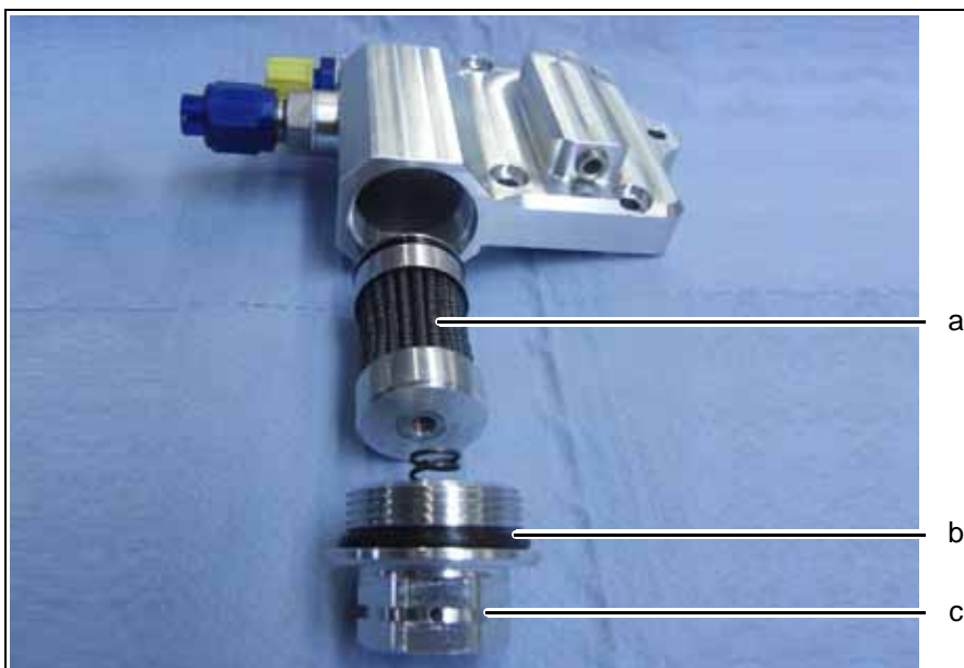
Fig. 6.14 Gearbox oil filter assembling
