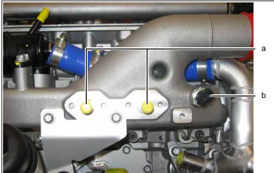
Fig. 6.5 Air temperature sensor and MAP connections of the intake manifold
