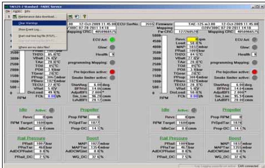
Fig. 6.38 FADEC read-out - Clear warnings
