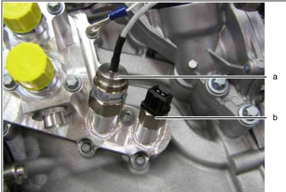
Fig. 6.11 Oil pressure- and oil temperature sensor
