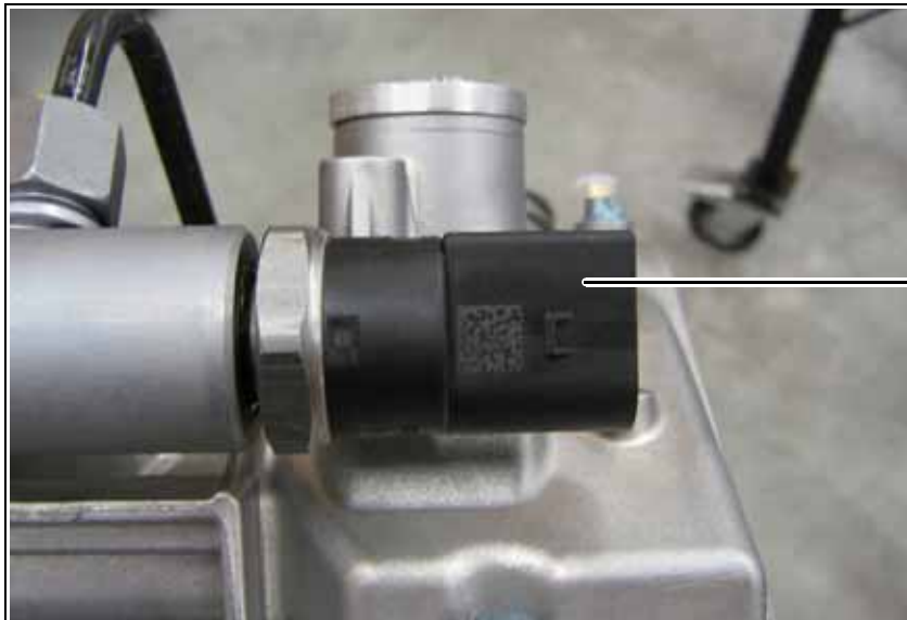
Fig. 6.4 Rail pressure sensor
