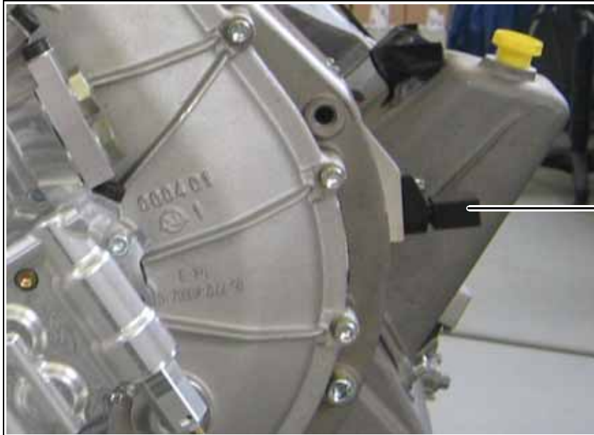
Fig. 6.9 Crankshaft sensor 2 a Crankshaft sensor FADEC B (2 of 2)
